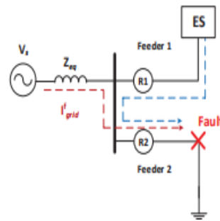
Fig2. Discharging of Energy Storage
