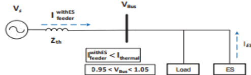
Fig 3. Feeder Level Integration.
