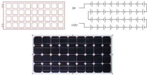
Fig 1. Illustration of solar module.
